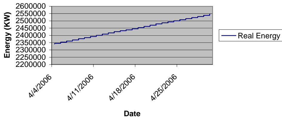
Real Energy Use - 480V - April
